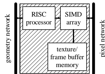
Figure 7: Simple block diagram of a PixelFlow node.
