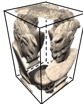
Figure 13. Object represented by six relief textures associated with the faces of a bounding box.
